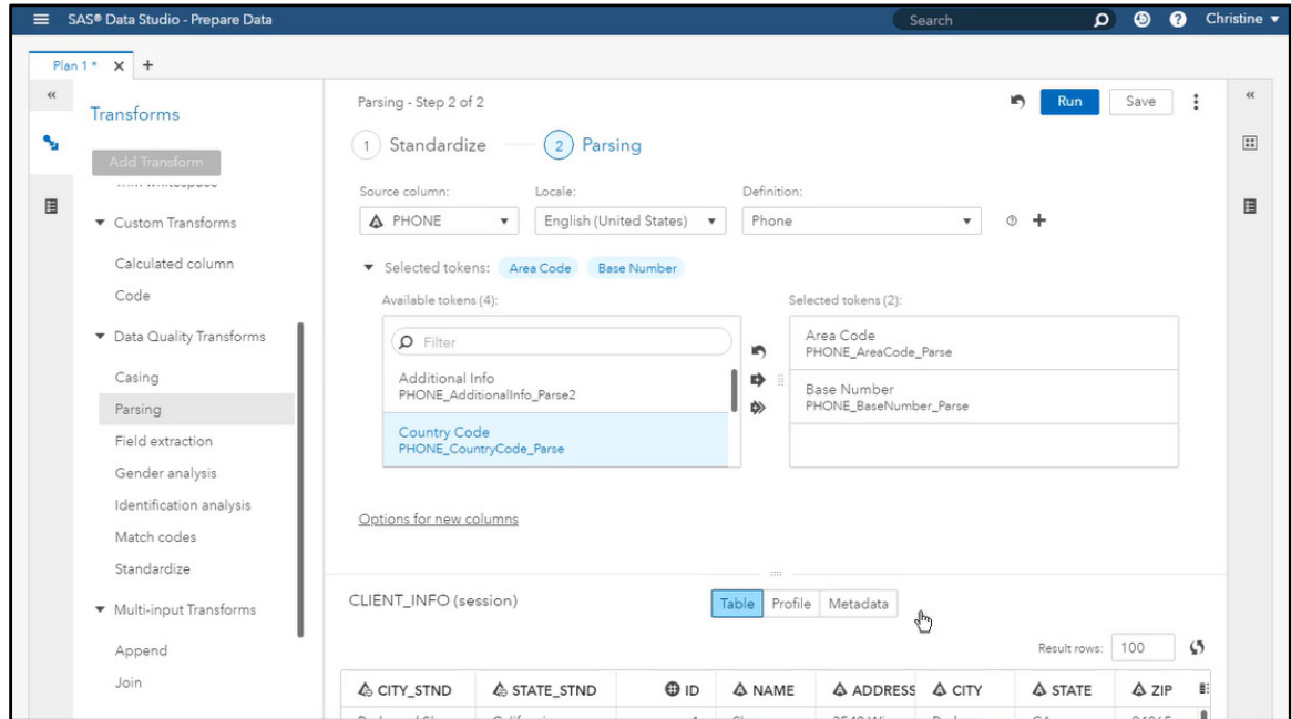
Figure 4.20: Parsing
