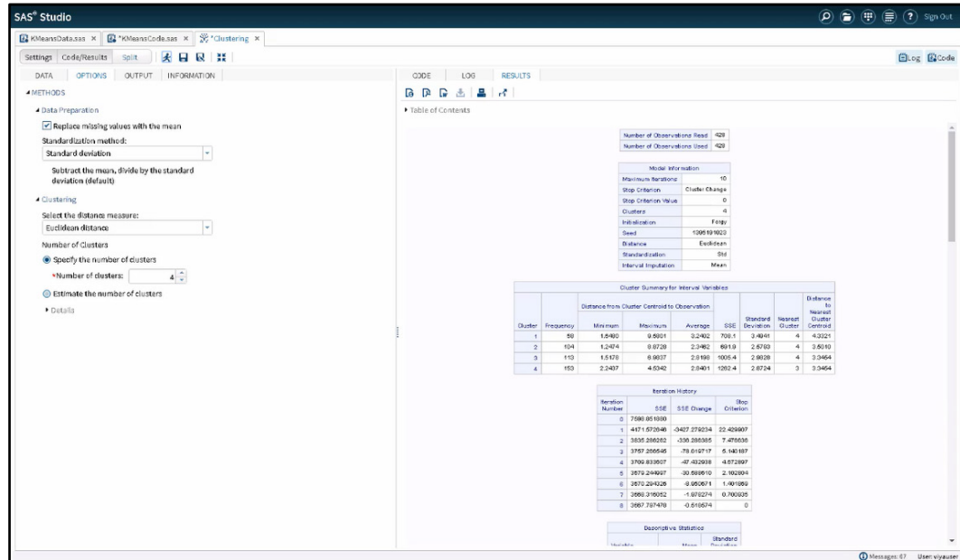
Figure 3.12: Clustering Results
